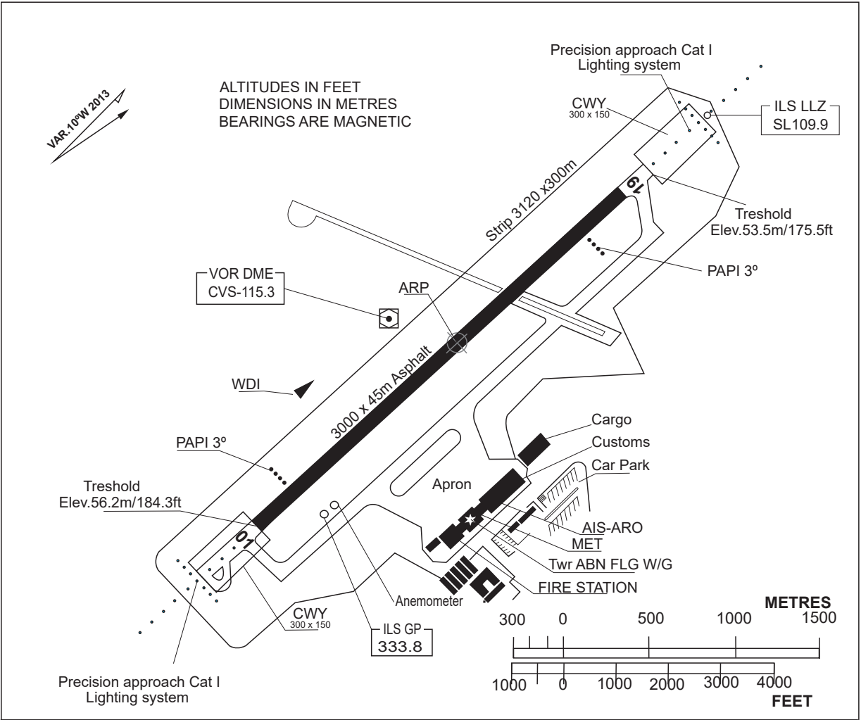
MARKING AIDS RWY 01/19 AND EXIT TWY
