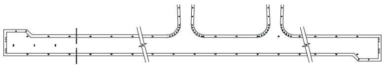
LIGHTING AIDS RWY 03-21 AND EXIT TWY
